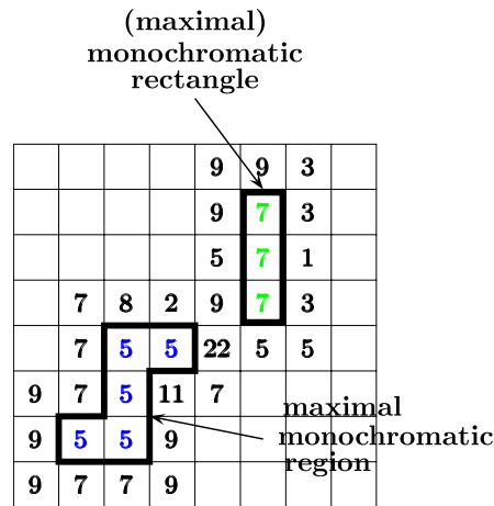
Fig. 1. An illustration of some communication-complexity definitions.
