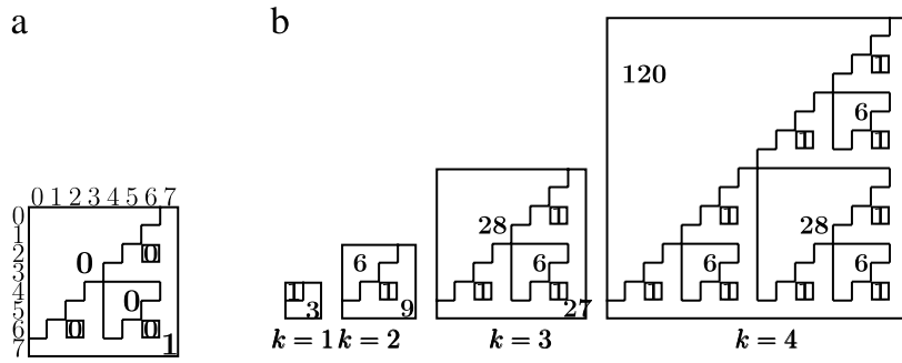
Fig. 11. (a) Ideal monochromatic partition for f_{\wedge, \vee} when k = 3 . (b) Sizes of ideal monochromatic partition for f_{\wedge, \vee} .
