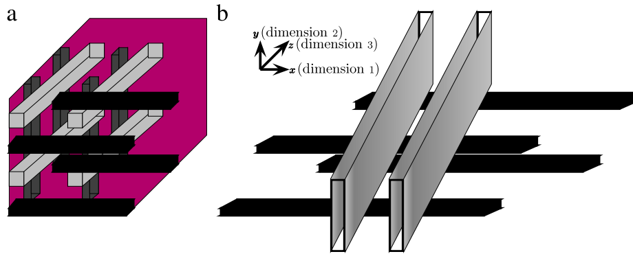
Fig. 9. (not drawn to scale) (a) The tiling function in the proof of Theorem 3. The non-trivial rectangles for dimensions 1, 2 and 3 are colored by black, dark gray and light gray, respectively; the trivial rectangles, each having a distinct value, cover the region colored magenta. (b) Rectangles (in light gray) corresponding to a hypothetically first meaningful step of the protocol.
