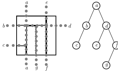
Fig. 7. BSP and Bsp-tree.
