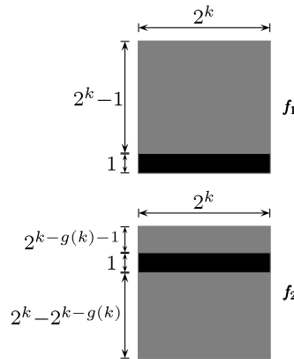
Fig. 4. This configuration cannot happen in Case 2.
