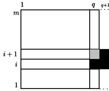
Fig. 4. This configuration cannot happen in Case 2.
