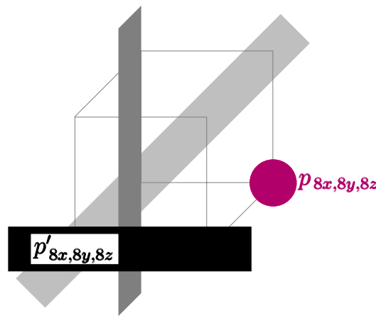
Fig. 10. Separating p_{8x,8y,8z} from p'_{8x,8y,8z} .
