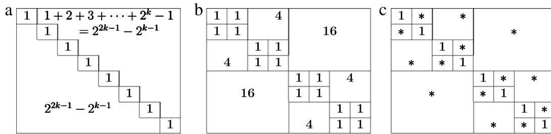
Fig. 13. (a) Ideal tiling for equality function. (b) The induced tiling by the bisection protocol (shown for k = 3 ). (c) Contribution of each rectangle in protocol-induced tiling where * \equiv 2^{2k-1} - 2^{k-1} . The numbers in the figure denote the size of each tile.
