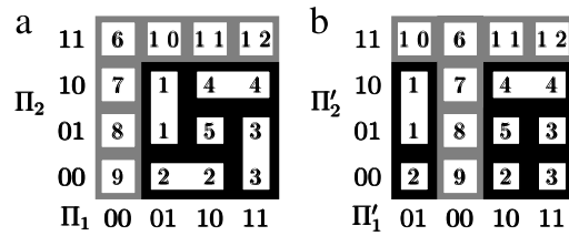
Fig. 2. A tiling function with respect to different permutation pairs (\Pi_1, \Pi_2) and (\Pi'_1, \Pi'_2) inducing different numbers of monochromatic rectangles.
