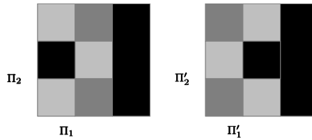
Fig. 3. Tilability depends on \Pi_1 and \Pi_2 .
