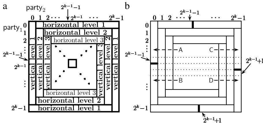
Fig. 8. Illustrations of the arguments in the proof of Theorem 2. The dotted lines in (b) are shown for visual clarity only.
